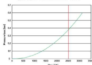
Typical pressure loss curve - R400
