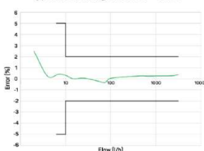
Typical metrological curve - R400
